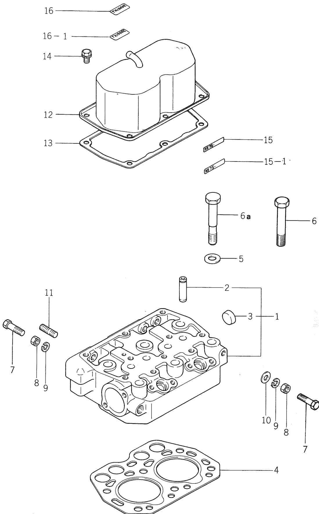
Fig. 1 CYLINDER HEAD Culasse
