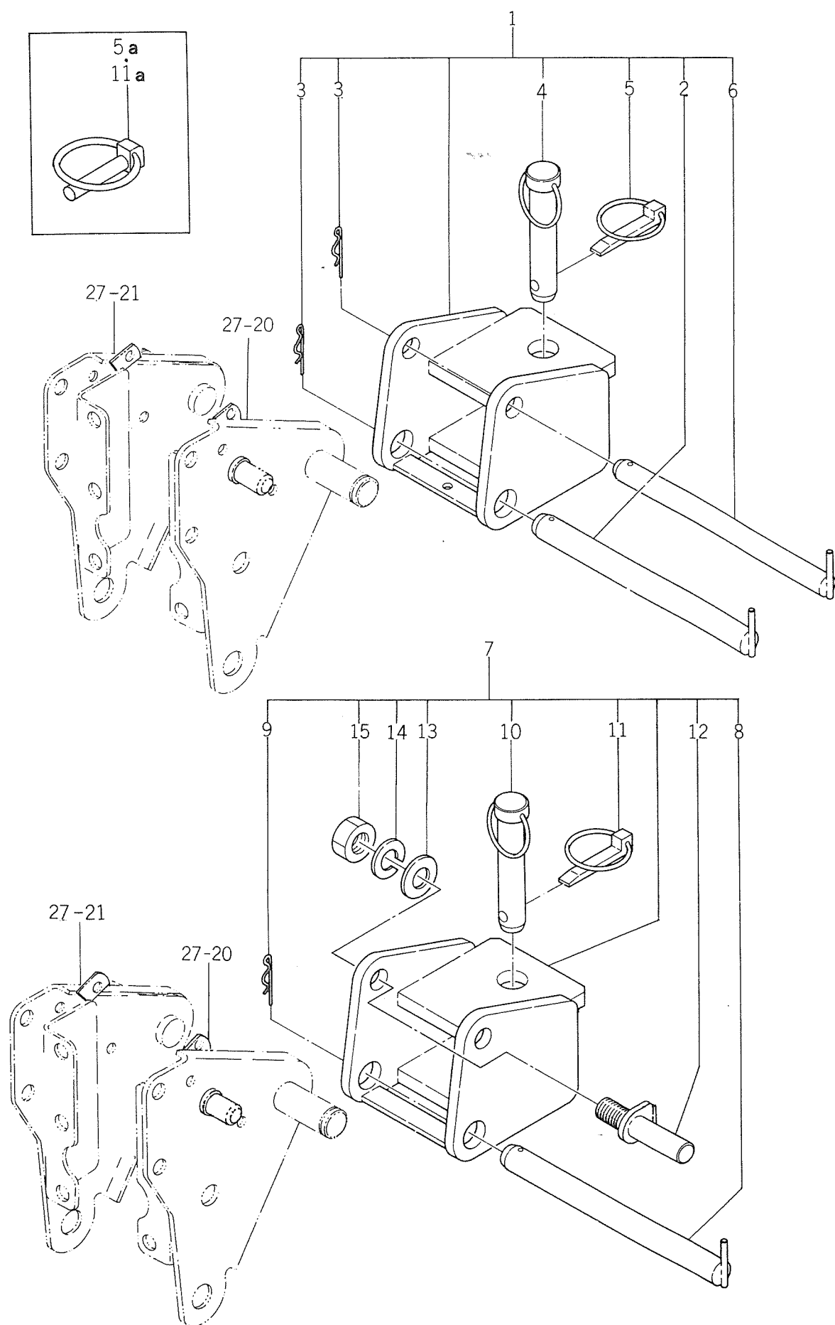
TRAILER HITCH
