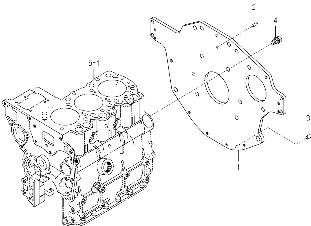
FIG. 8 REAR PLATE
