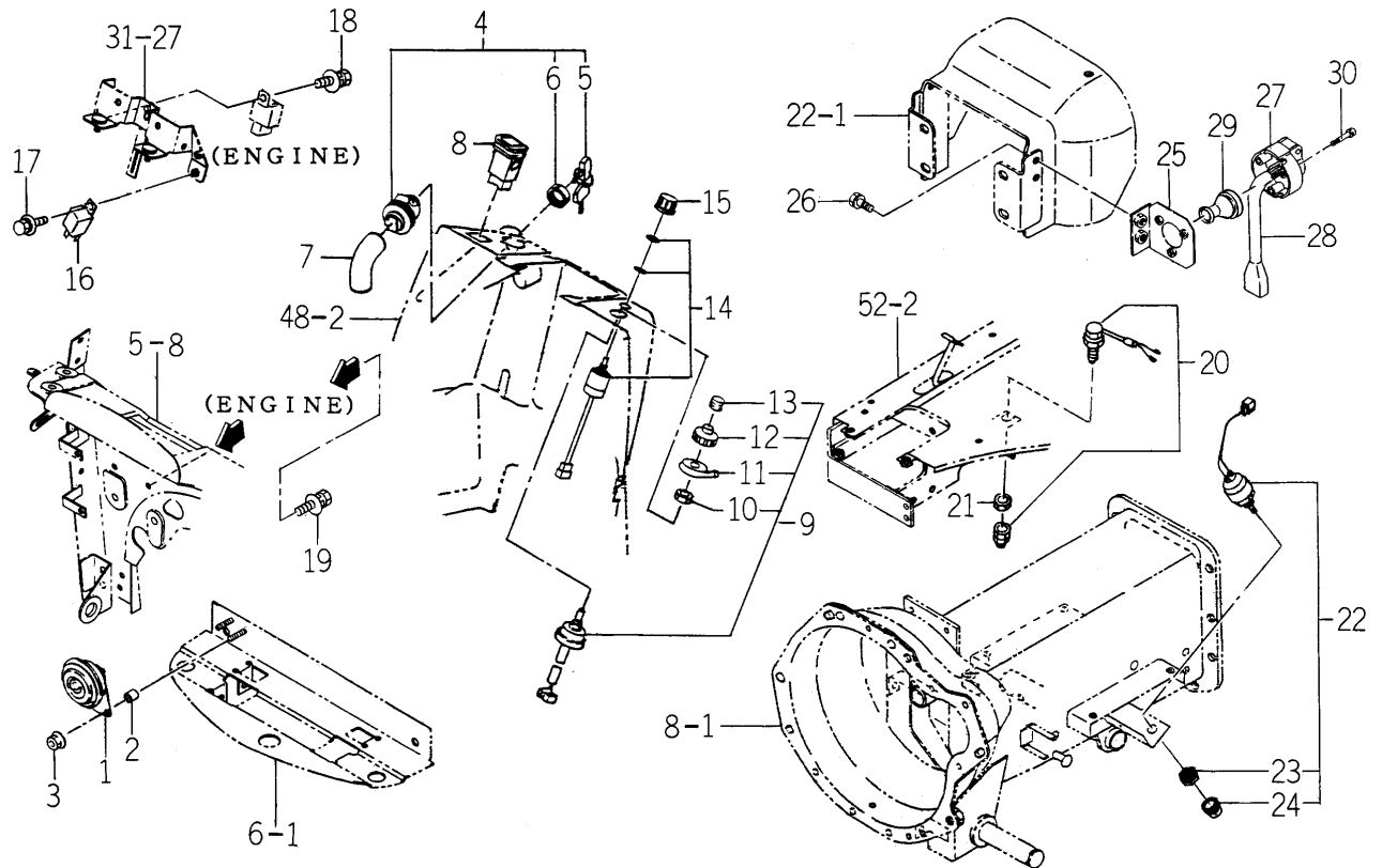
FIG. 55 SWITCH SYSTEM
