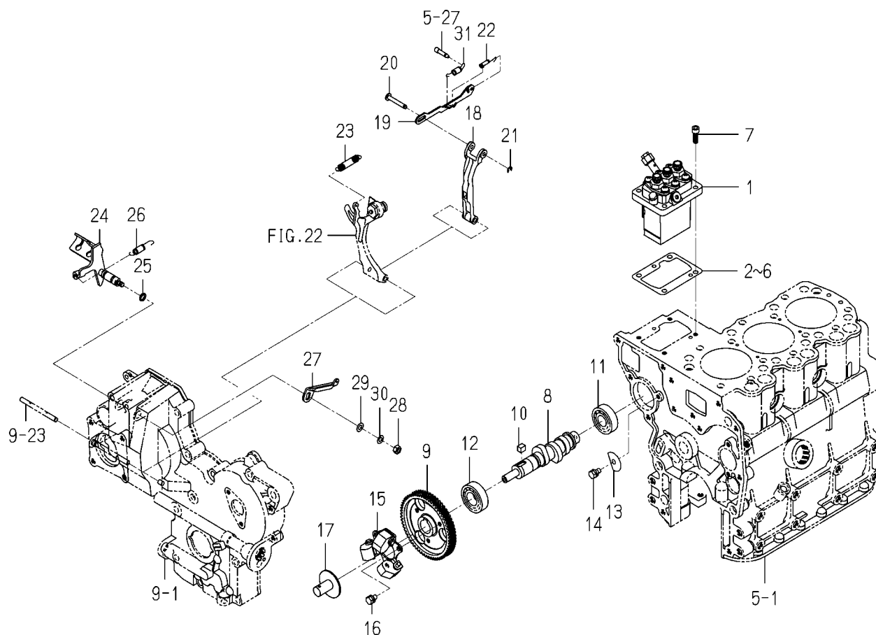
FIG. 20 INJECTION PUMP
