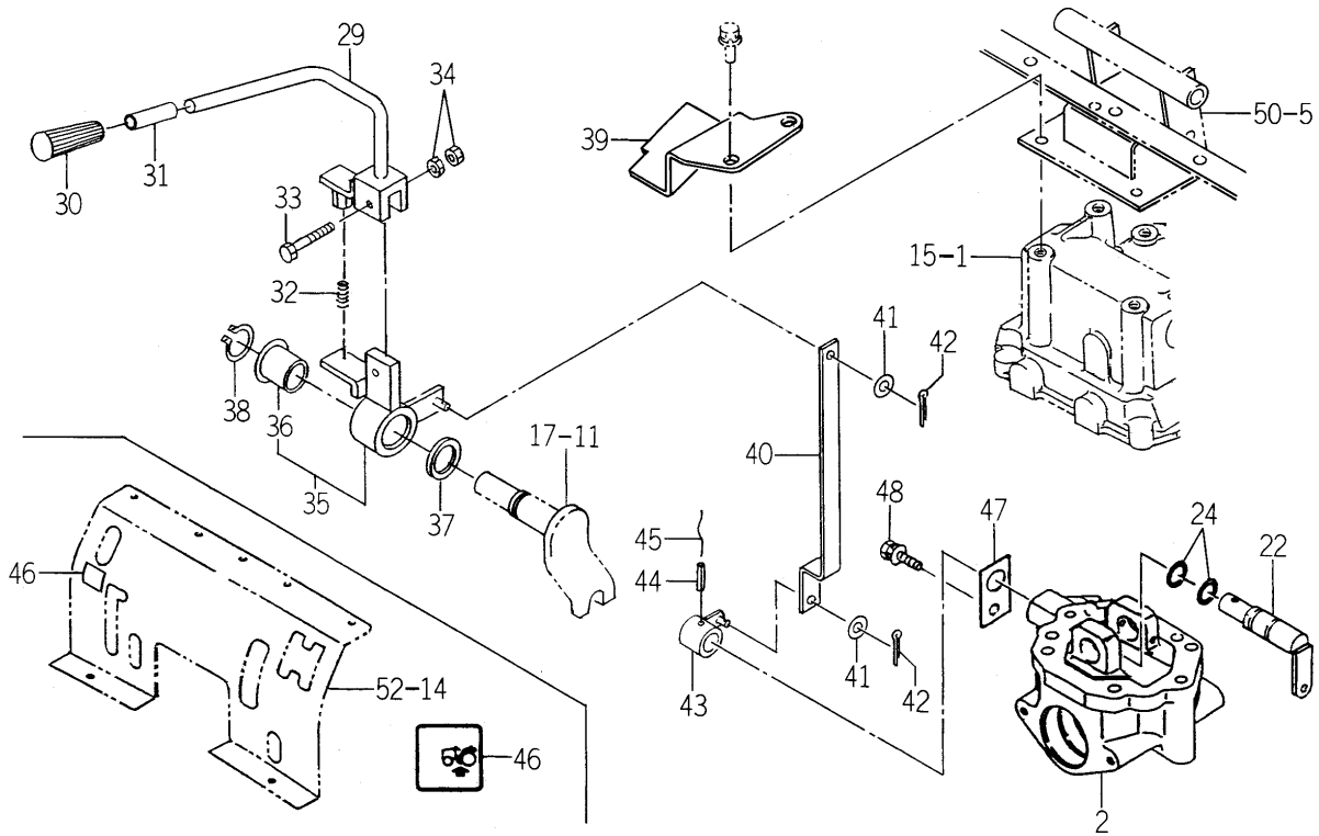
FIG. 62 MID PTO SET (EXCEPT M TYPE)(2/2) (OPTION)
