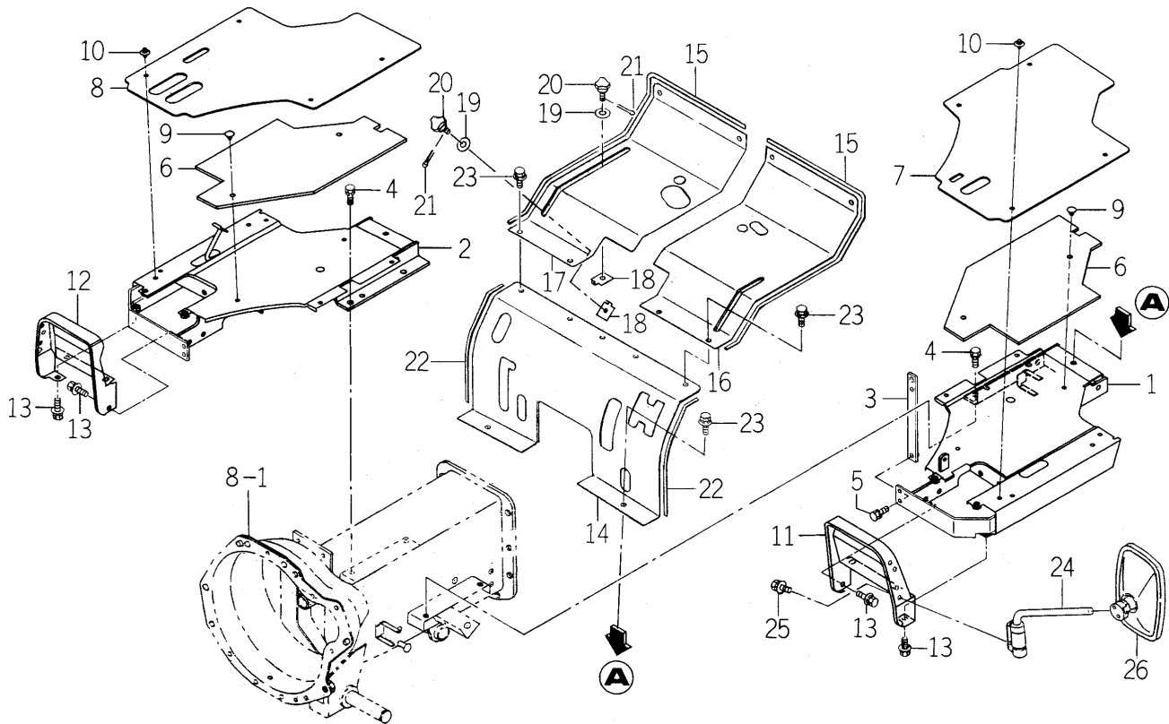
FIG. 52 STEP SYSTEM
