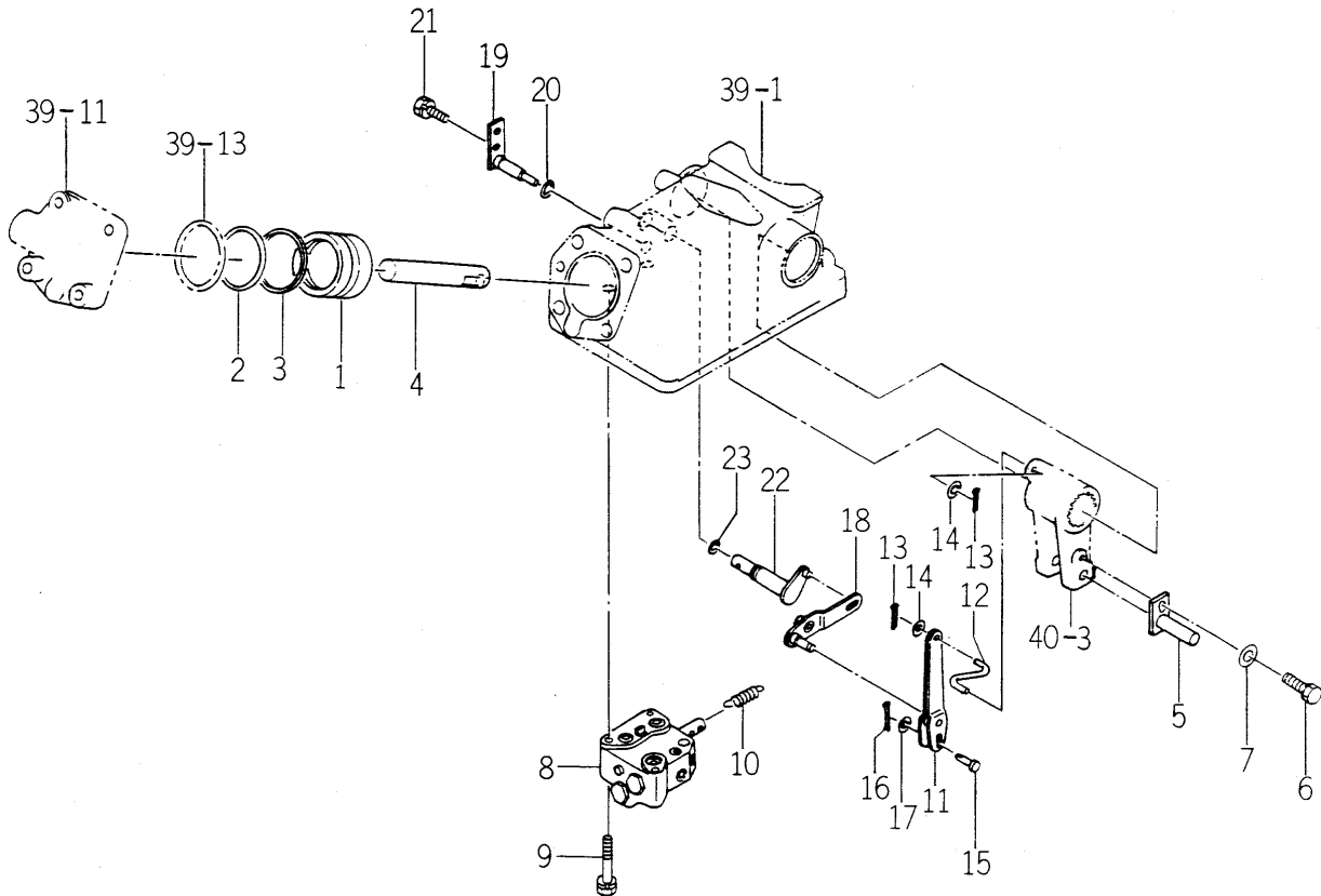
FIG. 41 CYLINDER SYSTEM
