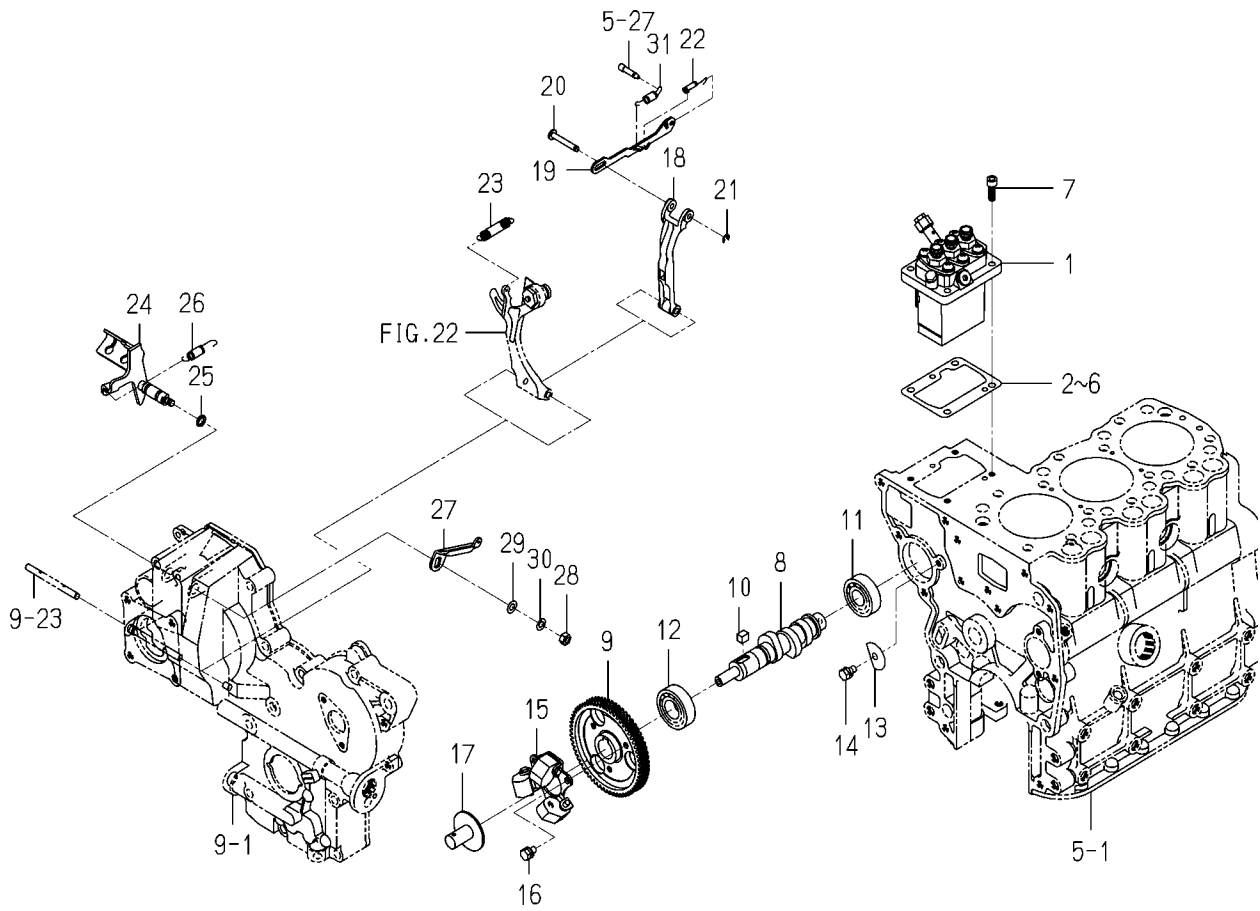
FIG. 20 INJECTION PUMP
