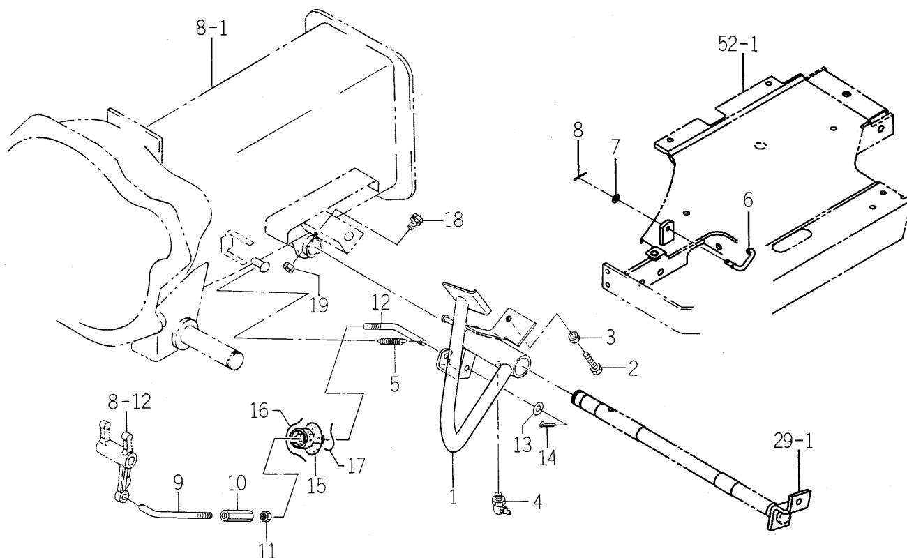
FIG. 9 PEDAL (CLUTCH) SYSTEM
