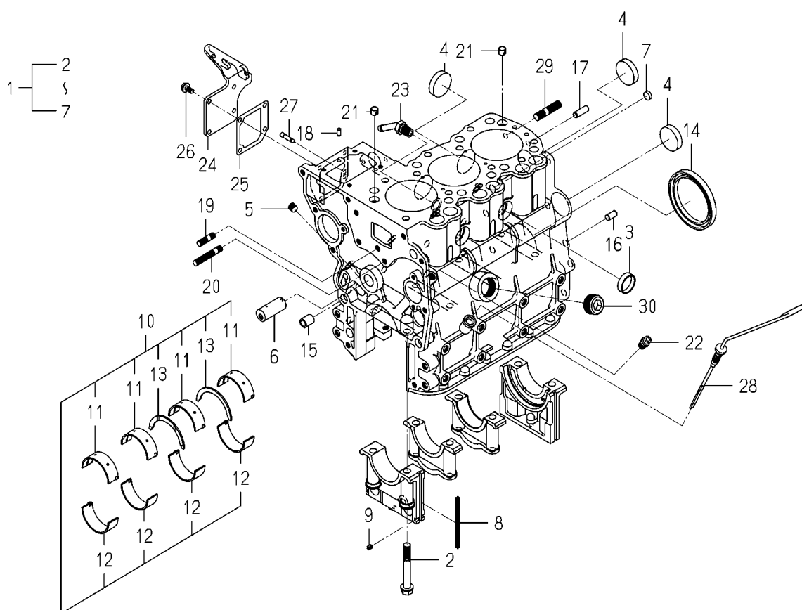
FIG. 5 CYLINDER BLOCK
