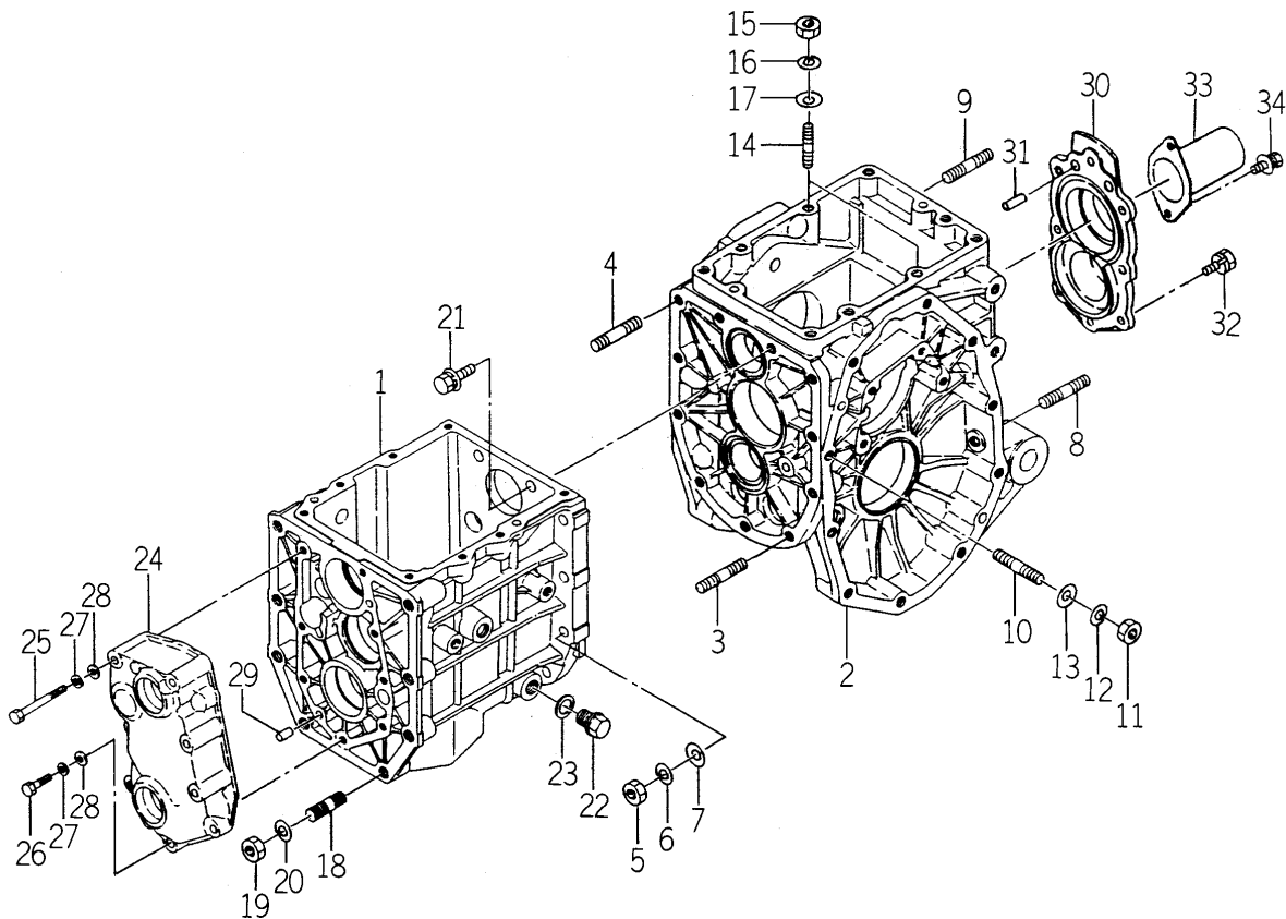
FIG. 10 CASE (TRANSMISSION) SYSTEM
