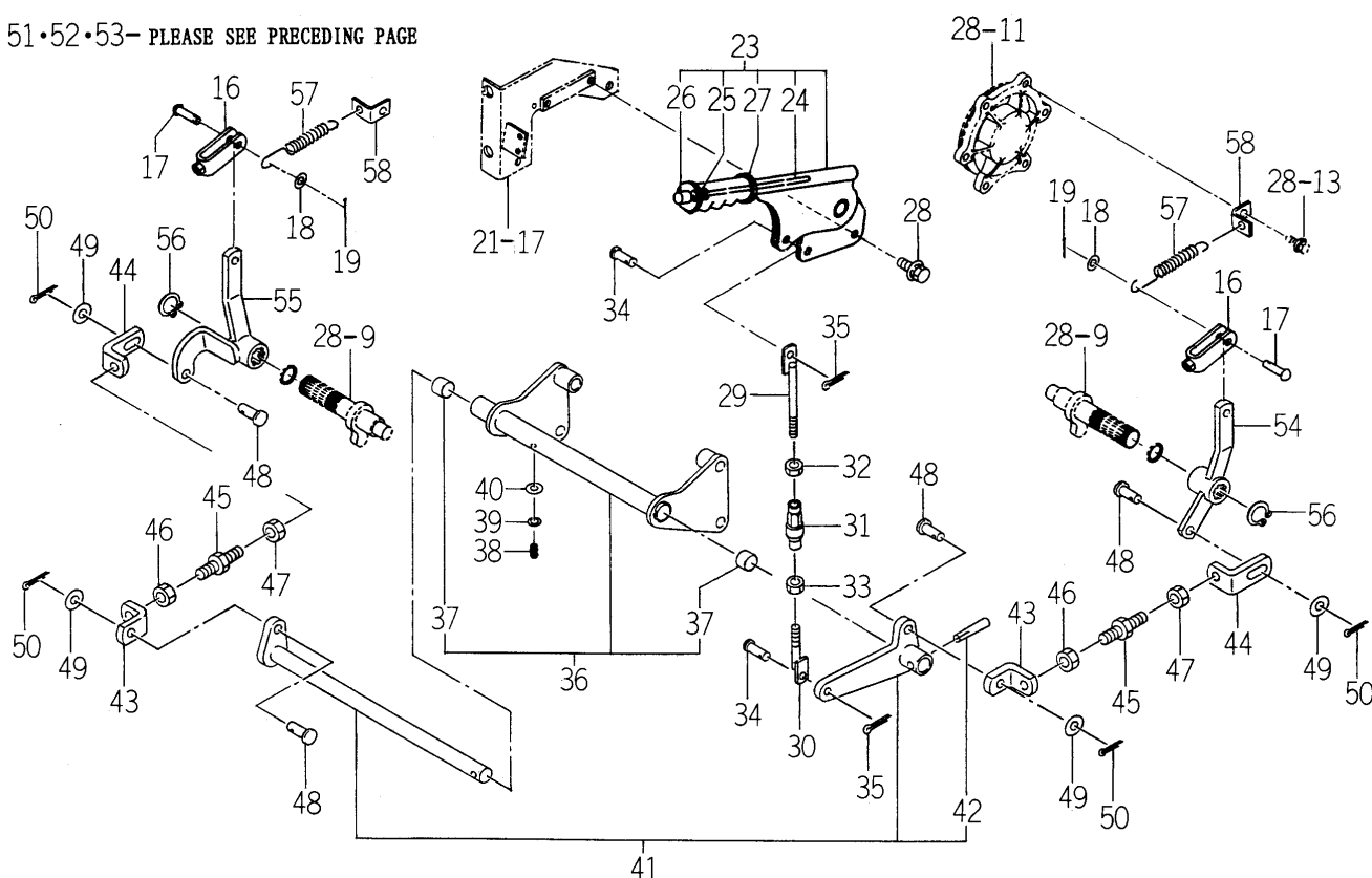
FIG. 29 PEDAL (BRAKE) SYSTEM(2/2)
