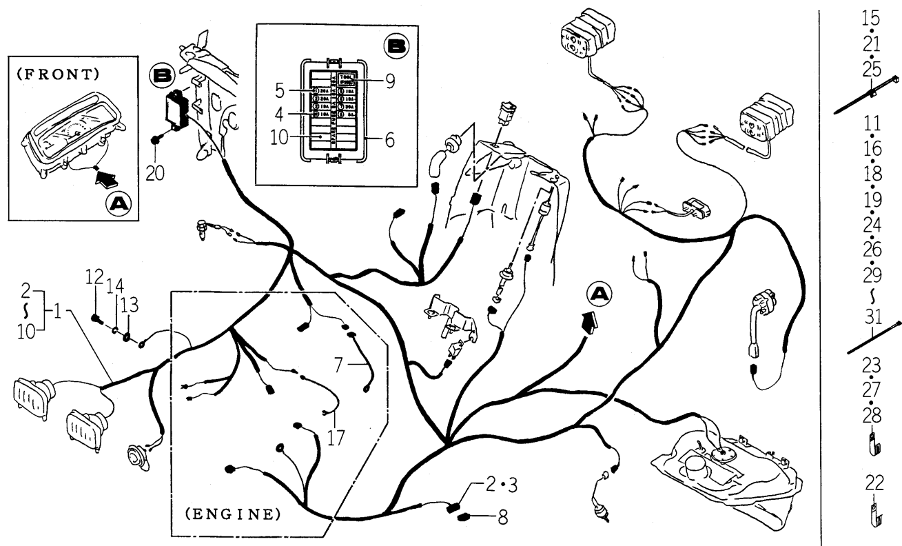
FIG. 56 HARNESS SYSTEM
