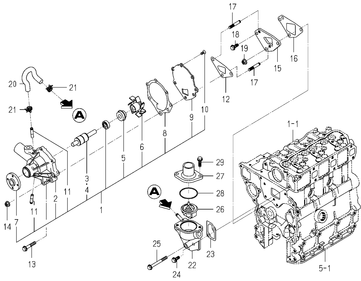
FIG. 17 WATER PUMP
