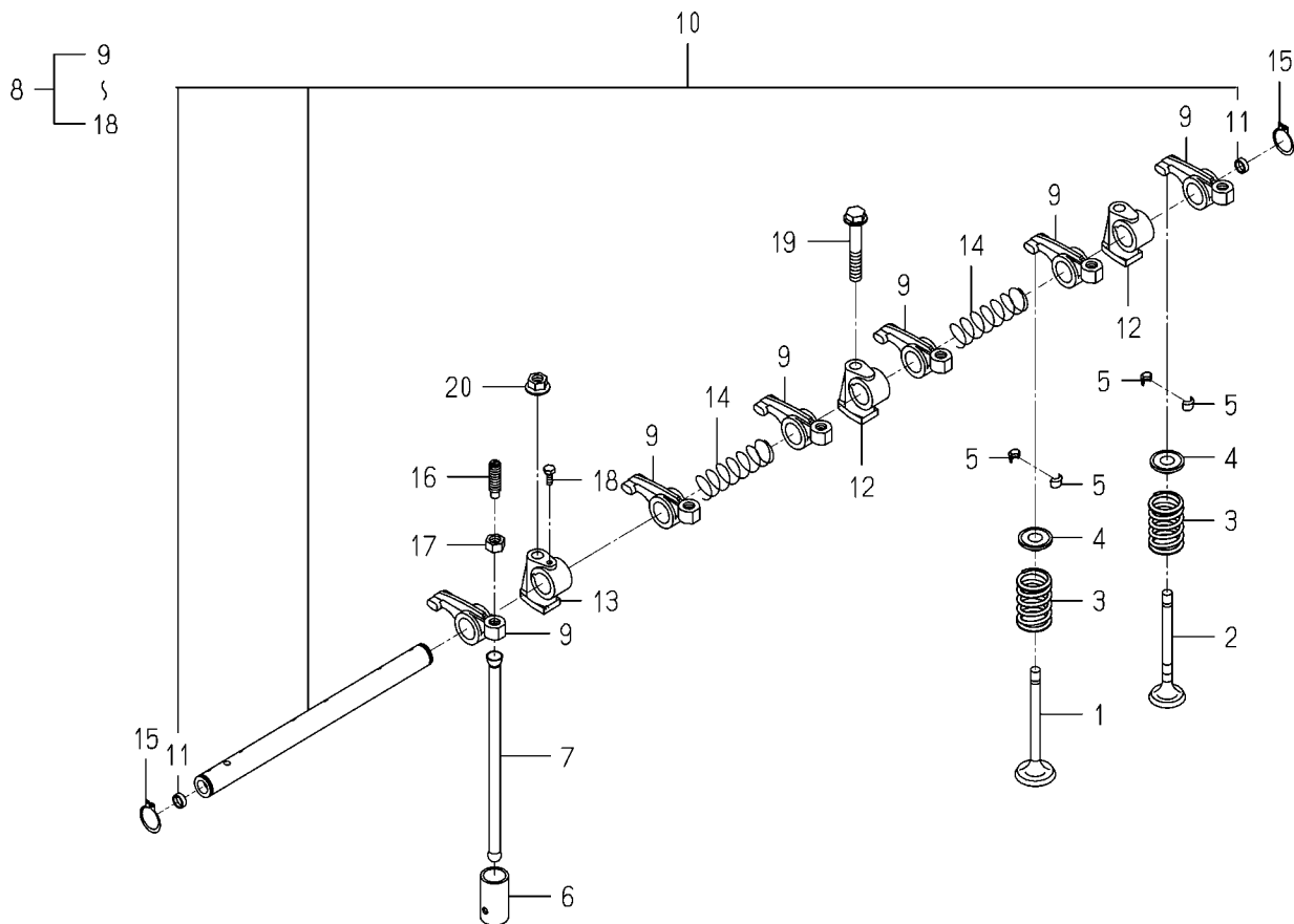
FIG. 11 VALVE
