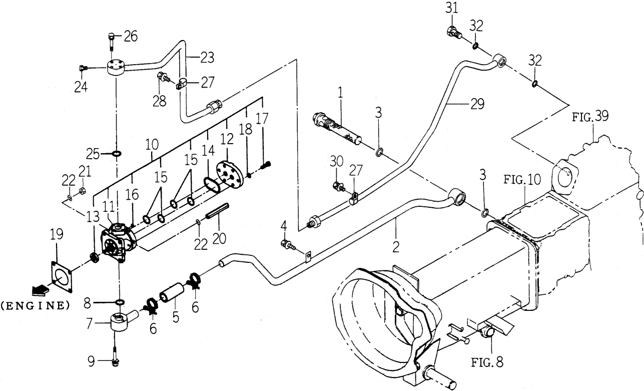
FIG. 43 PIPING SYSTEM
