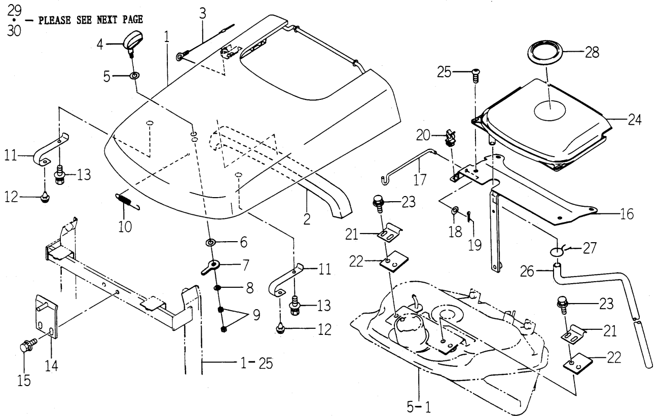
FIG. 46 HOOD SYSTEM(1/2)
