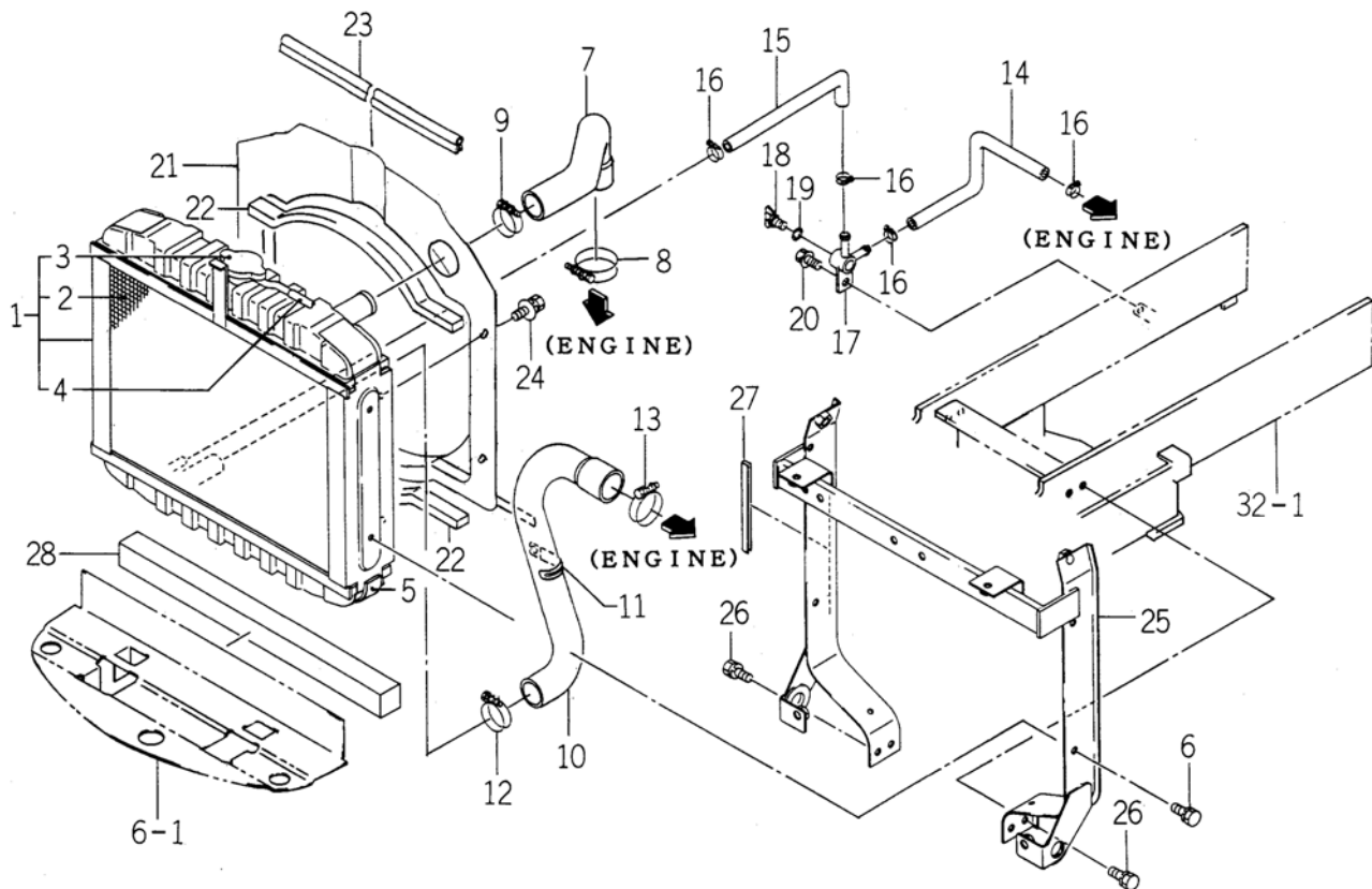
FIG. 1 RADIATOR SYSTEM
