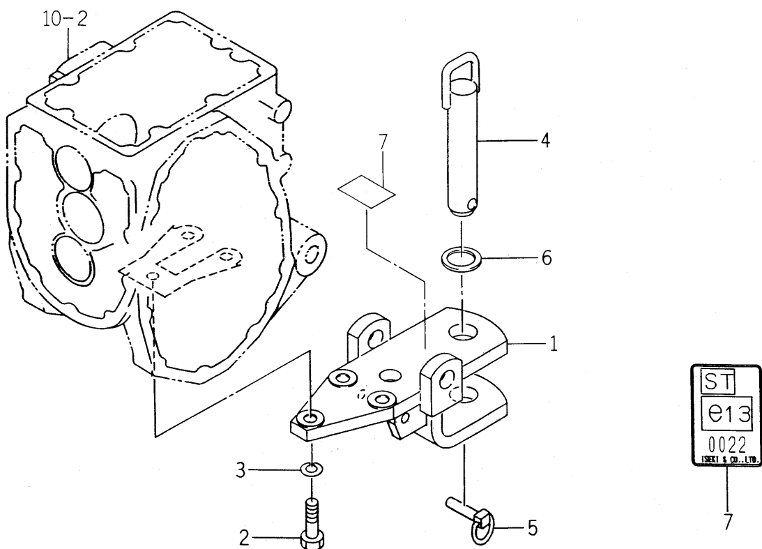
FIG. 45 HITCH (DRAW BAR) SYSTEM (R TYPE)
