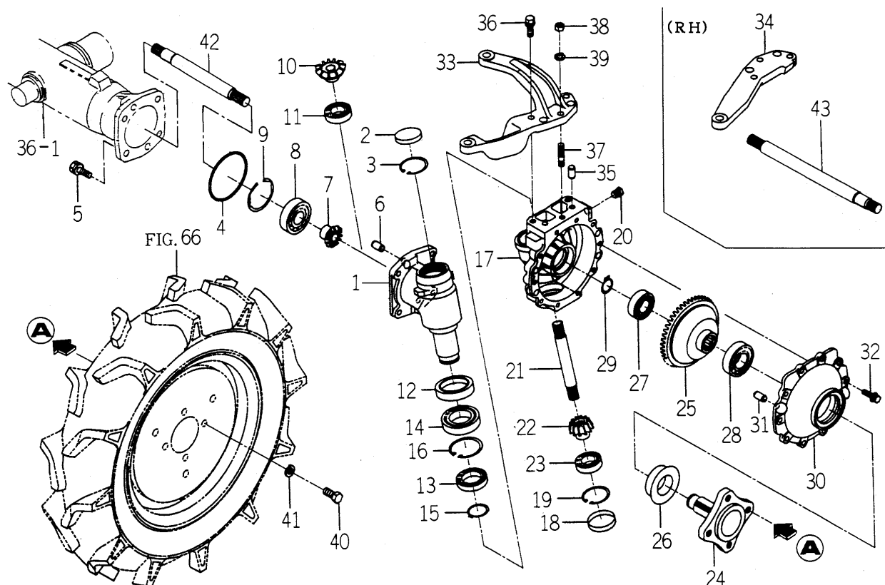
FIG. 37 FINAL GEAR CASE SYSTEM
