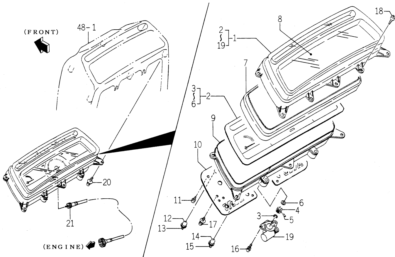
FIG. 54 PANEL SYSTEM
